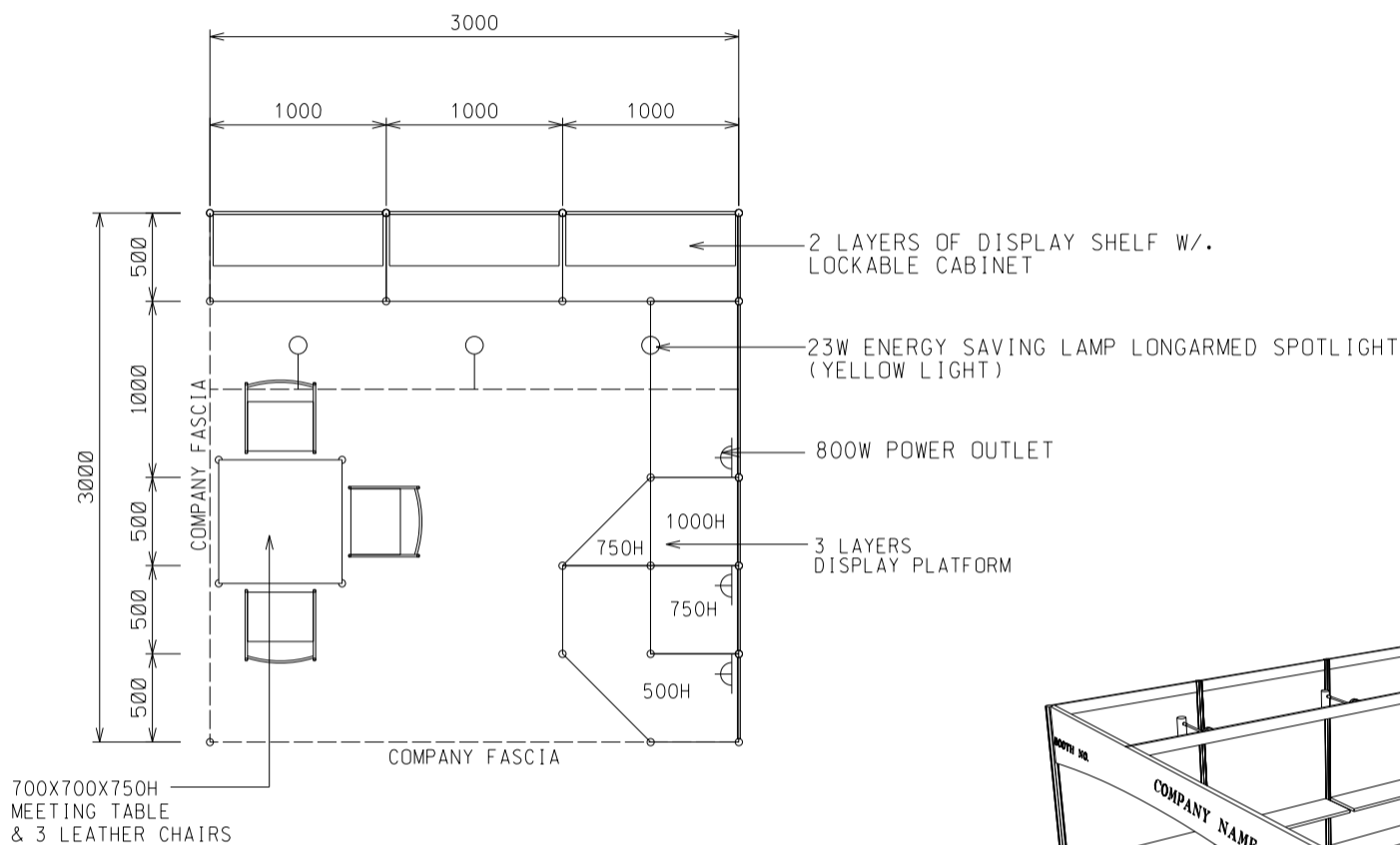
PLAN 3M(W) X 3M(D) X 2.5M(H) Left Corner Booth B
